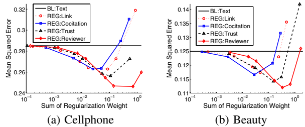
Figure 5: Parameter Sensitivity.
