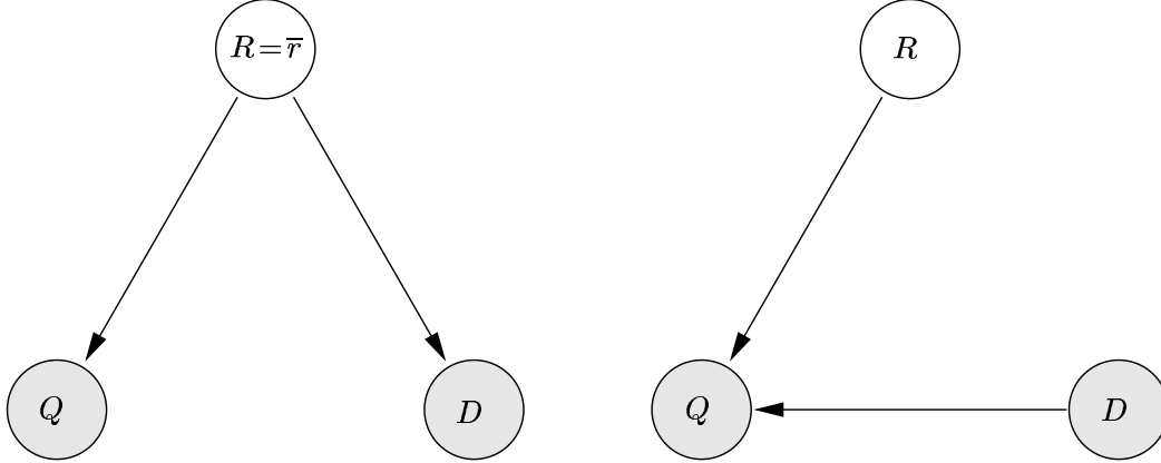
Figure 2: Graphical representations of the document-query distribution under Assumption 1 (left), and Assumption 2 (right).
