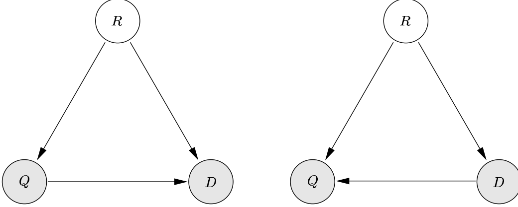
Figure 1: Graphical representations of the two factorizations of the joint document-query probability. The factorization p(D, Q | R) = p(D | Q, R) p(Q | R) (left) results in the Robertson-Sparck Jones model, while the factorization p(D, Q | R) = p(Q | D, R) p(D | R) (right) leads to the language modeling approach. Following convention, the document and query nodes are shaded to indicate that they are observed (“ this document and this query”).
