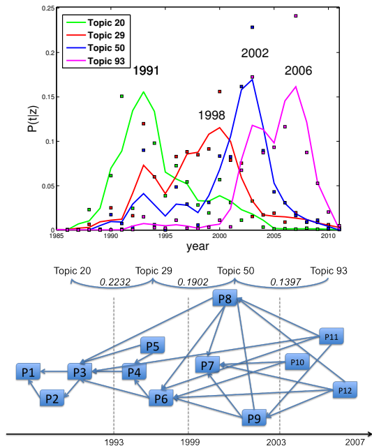
Figure 6: Temporal Evolution in Topics of Theme SMT
